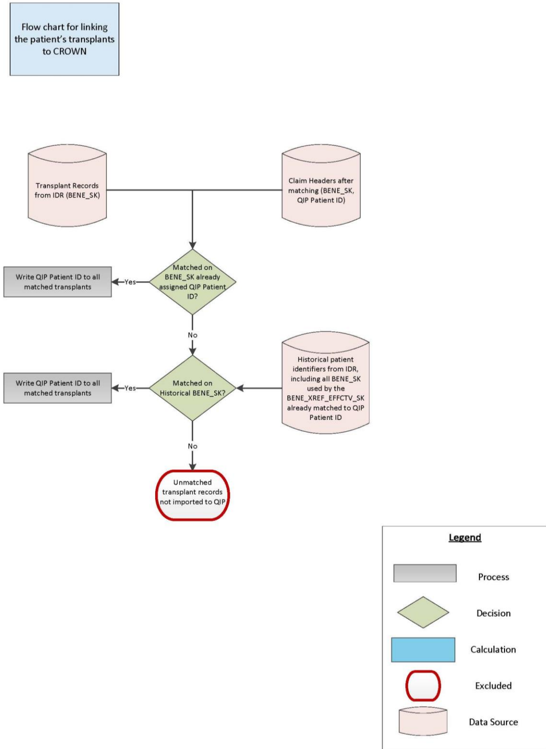
Figure 24: ESRD QIP Linking CROWNWeb Patients to Transplants
