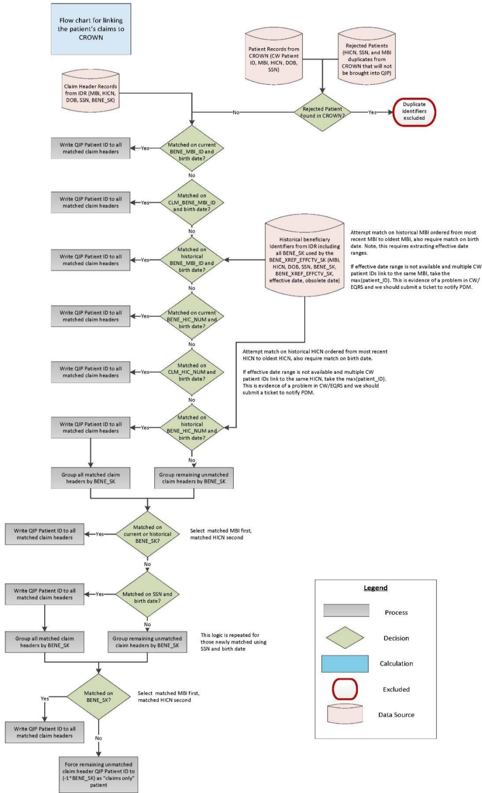
Figure 23: ESRD QIP Linking Claims and CROWNWeb
