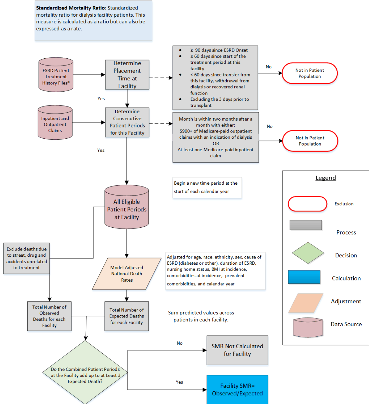
Figure 14: Standardized Mortality Ratio Flowchart (DFC Only)
